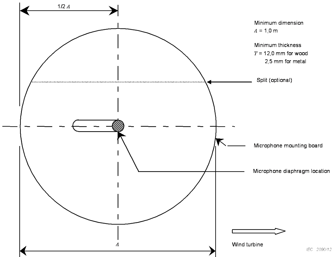
Figure 1a – Mounting of the microphone – Plan view
